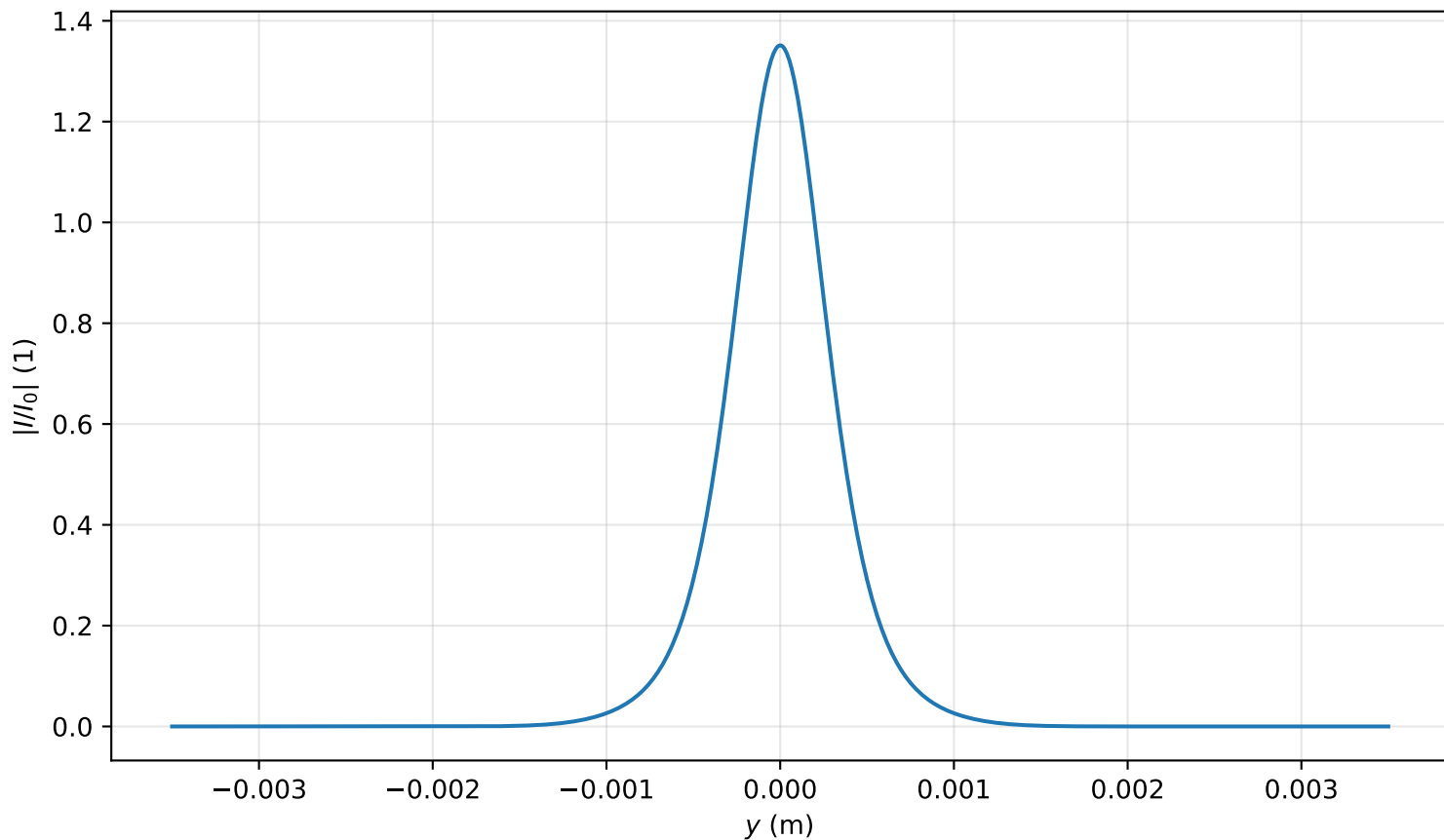
Intensity profile I(x=0, y, z=1.353)/I_0 , P_{in}=0.8P_{cr} , artificial time
